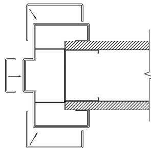
Example metal frame protection
