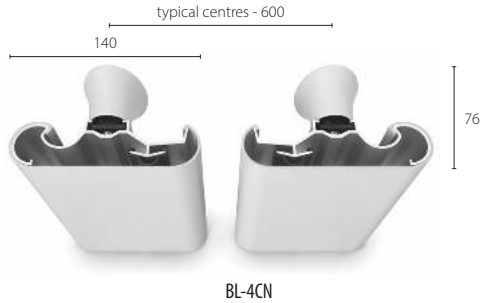
Quick Lock brackets are supplied in a colour matching cover.
