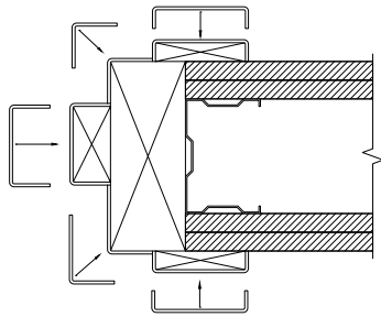
Example timber frame protection
