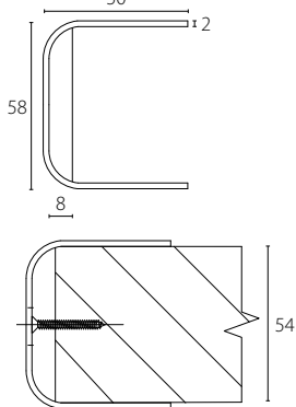
DE-06 (to suit 54 mm thick doors)
