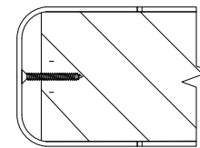
DEPs overlapping door face protection
