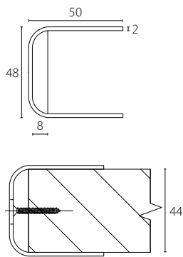
DE-01 (to suit 44 mm thick doors)
