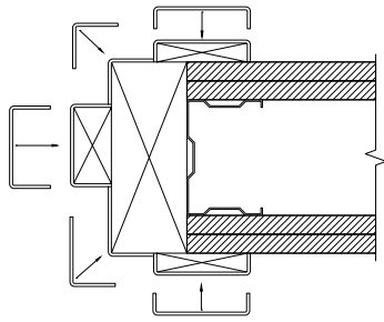
Example timber frame protection
