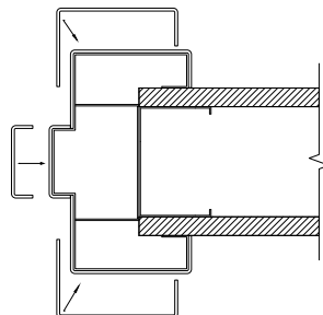
Example metal frame protection
